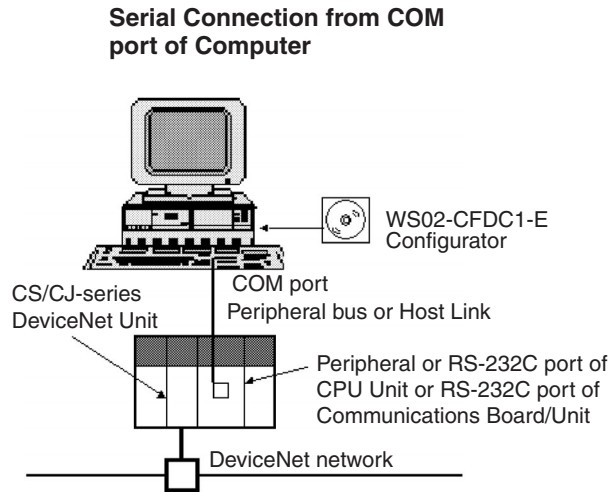
The Configurator is not treated as a single DeviceNet Node.
