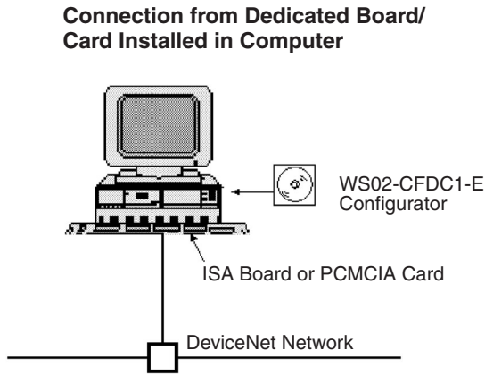
The Configurator is treated as a single DeviceNet node.
